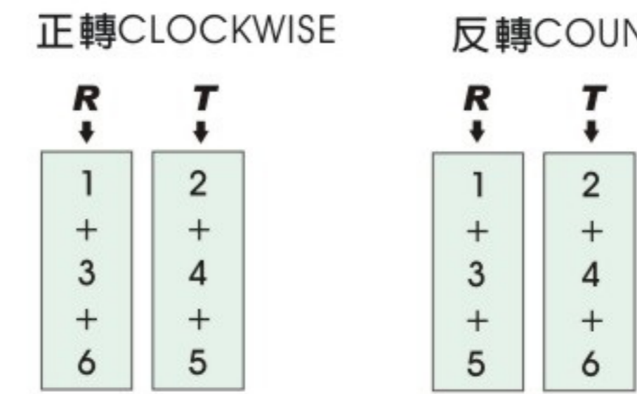
(a) 單相低壓 LOW VOLTAGE-110V
