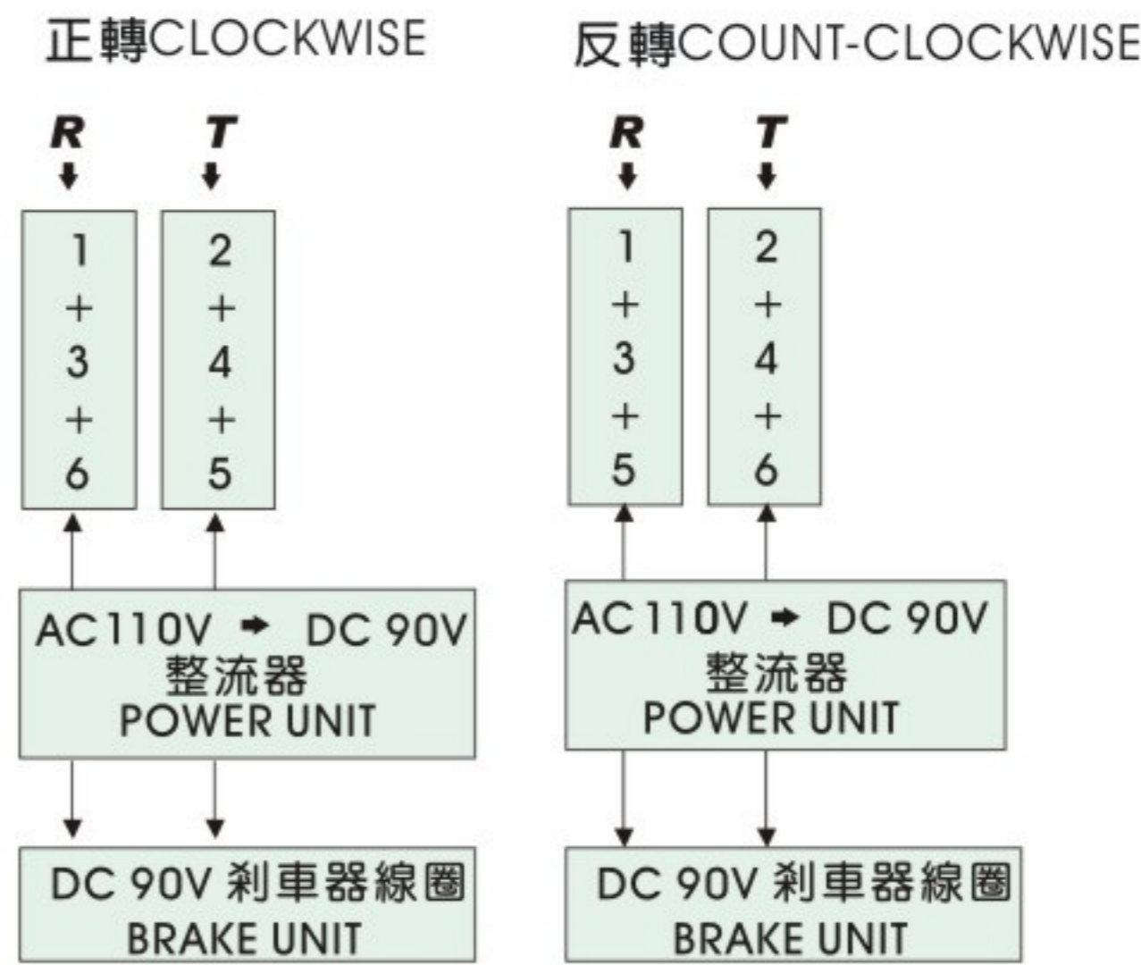
(c) 單相低壓110V附直流剎車器 LOW VOLTAGE 110V WITH DC BRAKE UNIT
