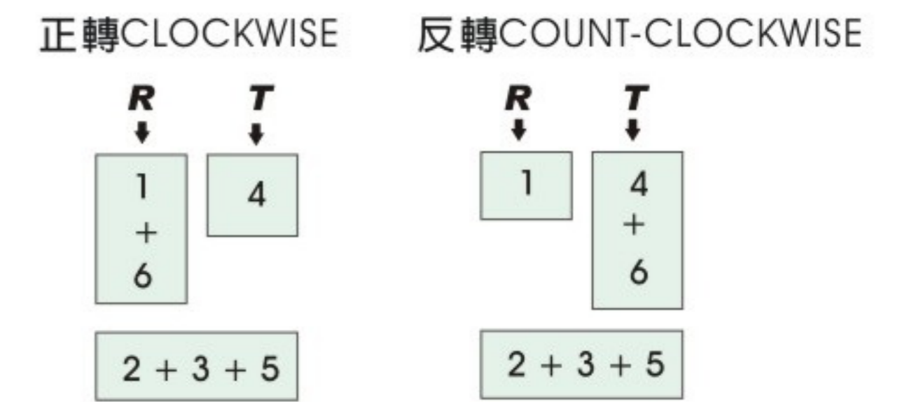
(b) 單相高壓 HIGH VOLTAGE-220V
